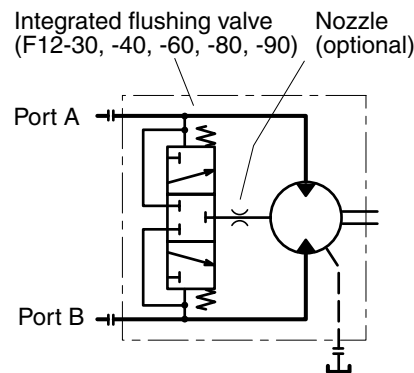
Hydraulic schematic.
