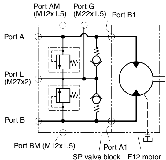
SP/F12 schematic.
